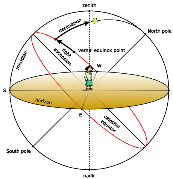
Figure G.2: Right Ascension & Declination
