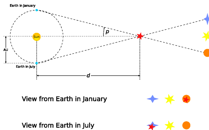
Figure G.6: Apparent motion due to parallax
