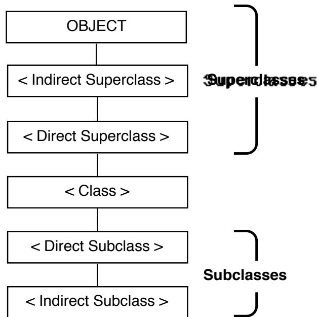
Fig. 1.2 Class Relationships
